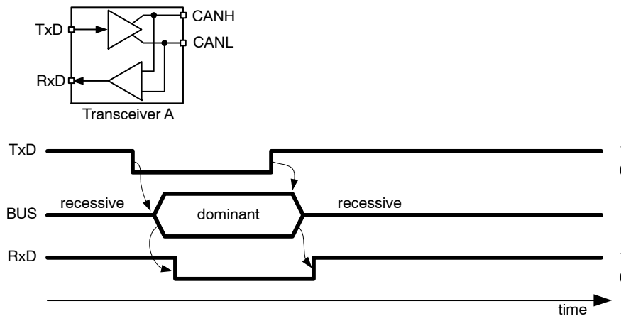
Figure 1. Simplified Model and Timing of a High-speed CAN Transceiver
