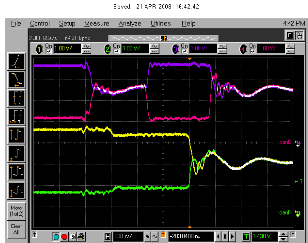
Figure 10. Signal repetition in case different nodes coincidentally transmit on both branches. Yellow and green – bus voltage on bus1; blue and magenta – bus voltage on bus2. Overall view and zoom on the transition dominant→recessive.
