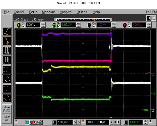
Figure 10. Signal repetition in case different nodes coincidentally transmit on both branches. Yellow and green – bus voltage on bus1; blue and magenta – bus voltage on bus2. Overall view and zoom on the transition dominant→recessive.
