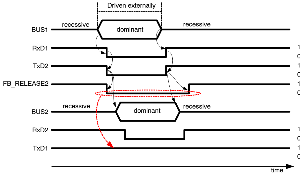
Figure 5. Signal Repetition Without a Deadlock Thanks to the Feedback Suppression
