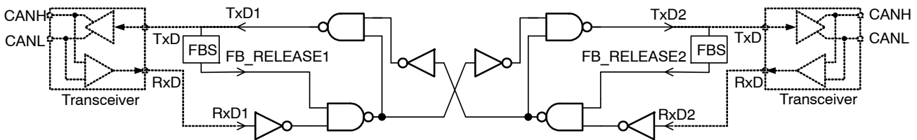
Figure 3. Repeater Logic with Feedback Suppression (FBS) used in AMIS42700 (simplified)
