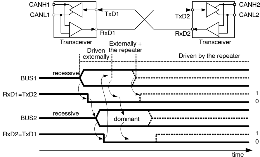
Figure 2. Direct Connection of 2 Transceivers and the Occurrence of a Deadlock on the Bus
