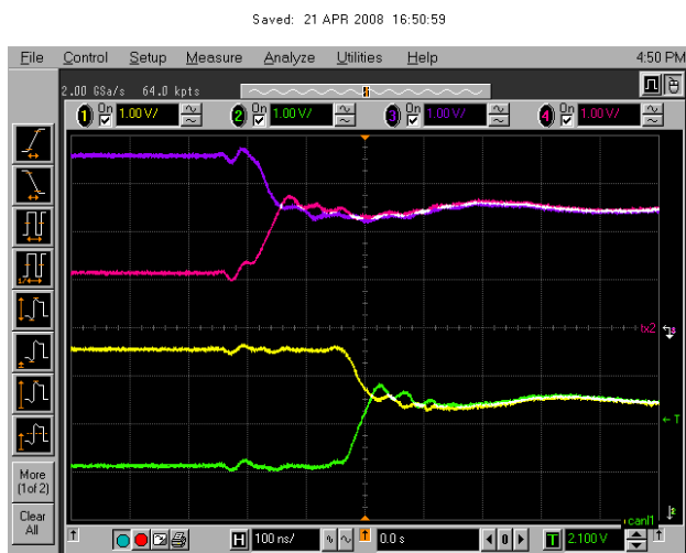
Figure 8. Signal repetition from CAN bus 2 (blue+ magenta) to CAN bus 1 (yellow + green) in case only one node transmits on bus1. Zooms to both signal transitions
