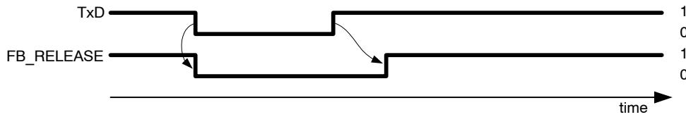
Figure 4. Function of a Feedback Suppression Block (FBS)
