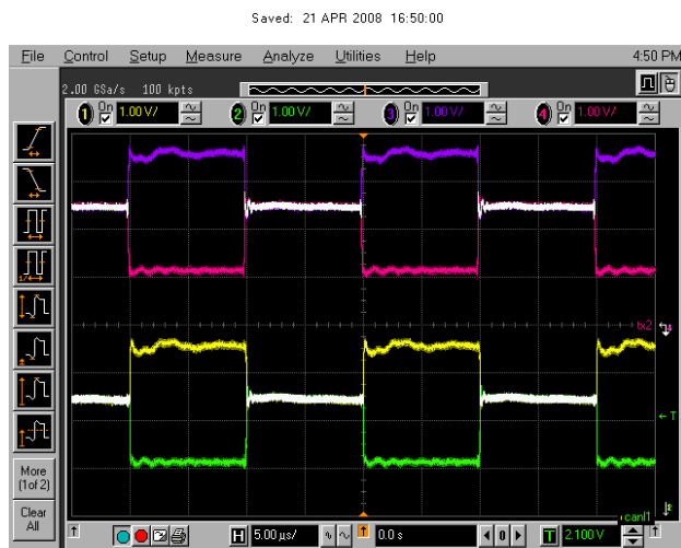
Figure 7. Signal repetition from CAN bus 2 (blue+ magenta) to CAN bus 1 (yellow + green) in case only one node transmits on bus1.
