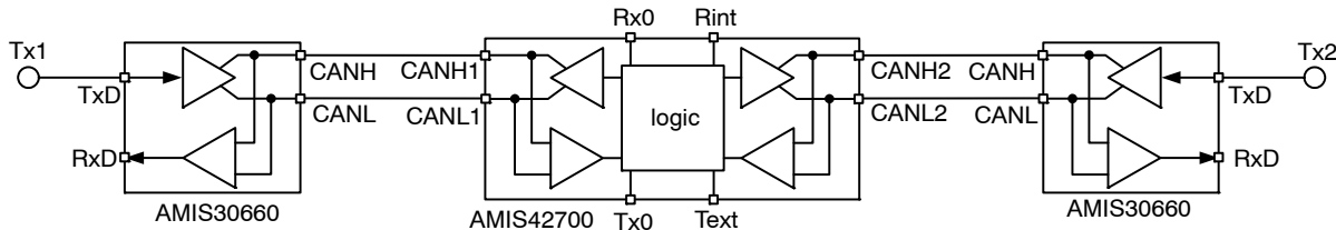
Figure 6. Measurement setup used to verify the repeater logic of AMIS42700 – bus terminations, common-mode chokes and other components are not depicted.
